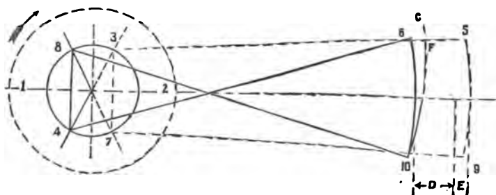
FIG. 289 —Diagram of the Operation of the Link Motion. The centres of the two eccentrics being at 4 and 8, the crank pin at 2, the link at mid-gear, the eccentric rods will be indicated by the full lines, 4-6, 8-10. When the crank pin is at 1, the centres of the eccentrics will be at 8 and 7, and the positions of the rods on the dotted lines, 3-5 and 7-9. The distance, D, indicates the vertical distance between the centres of the eccentrics in the full and dotted-line positions. If from the centre, 8, with the rod as the radius, an arc be drawn to F, the distance, C, shows the position of the link if both rods were "open" with the crank at the cylinder end, 2, instead of at the opposite dead centre, 1. The distance, C, is equal to the distance, E, and the total distance (D + E) that the valve moves is twice the lap, plus twice the lead, plus the distance, or angularity, occasioned by the rods being crossed, when the crank is on the cylinder end dead centre, 2, becoming opened when the crank is at dead centre, 1.
